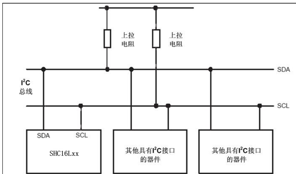
Figure 26-1 I 2 C 总线配置
