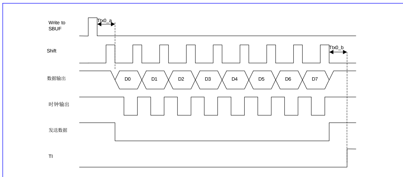
Figure 24-2 串口发送模式0
