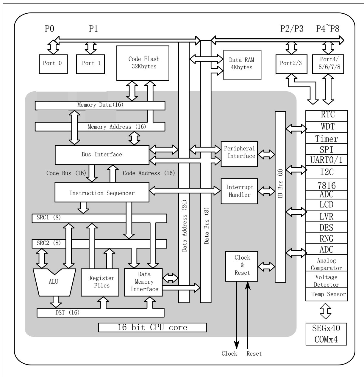
Figure 7-1 HC16Lxx CPU 模块
