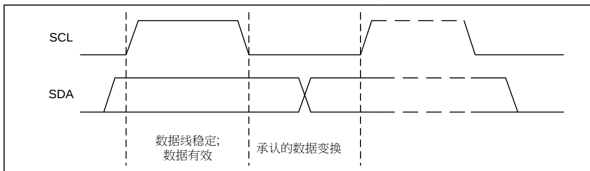
Figure 26-6 I²C 总线上位传输
