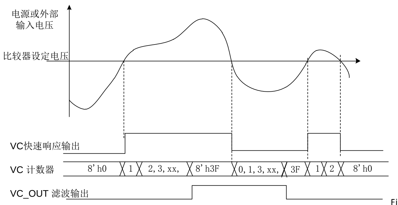
Figure 29-2 滤波响应时间
