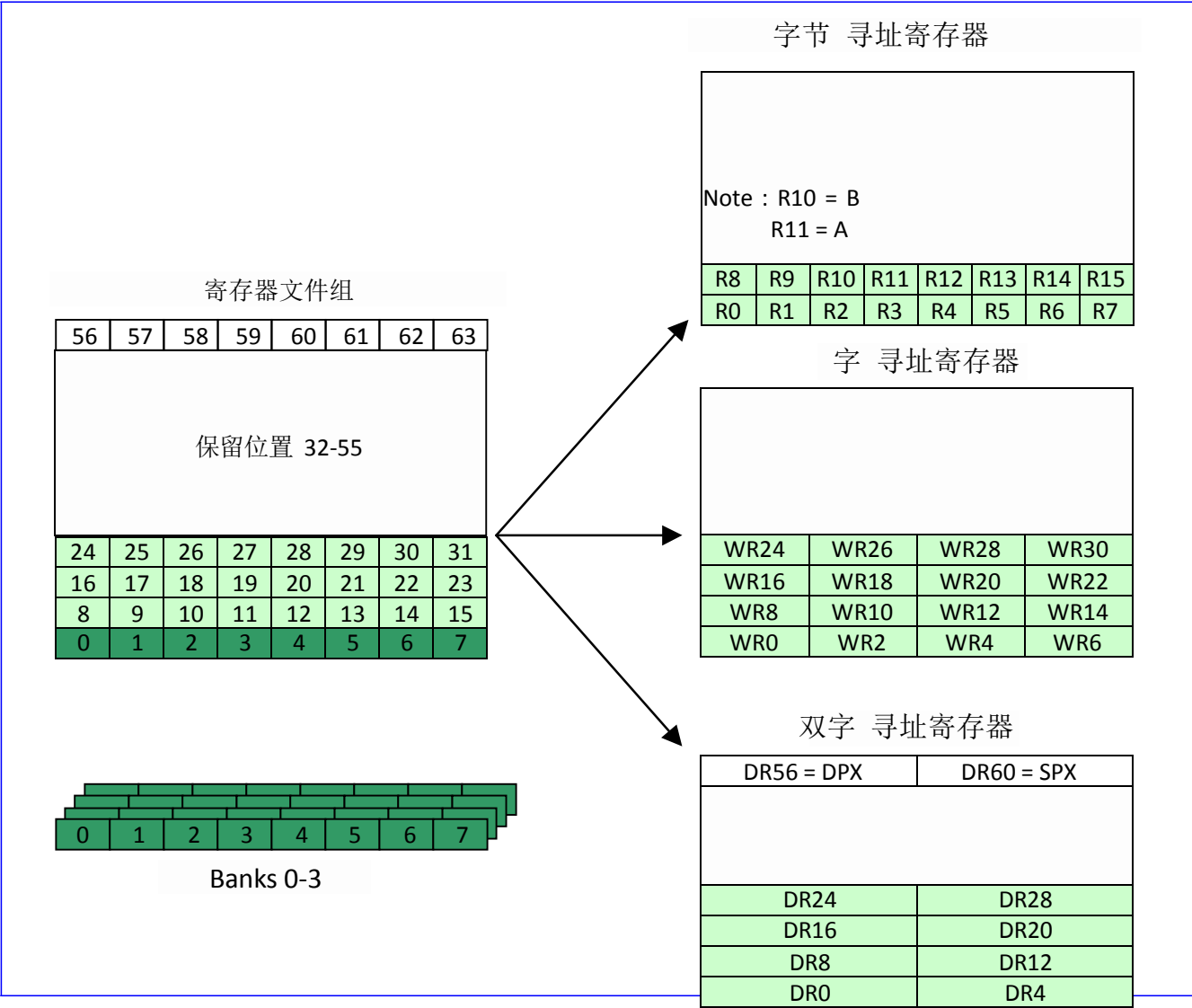
Figure 7-8 寄存器文件组
