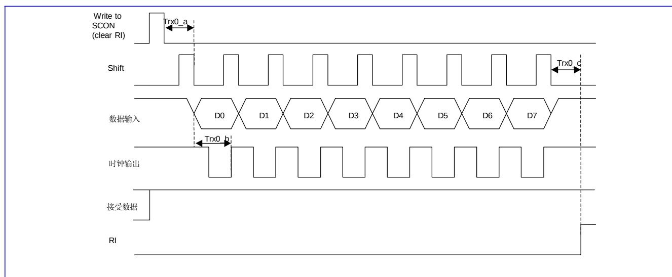
Figure 24-3 串口接收模式0
