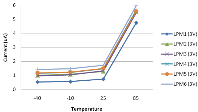
LPM1~LPM6 Temp & Current
