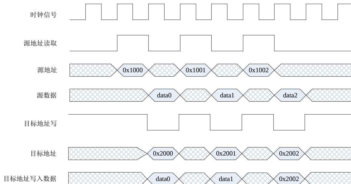
Figure 11-2 DMA 串行操作时序图
