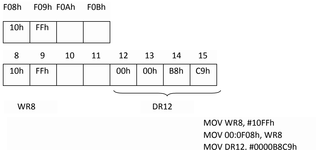
Figure 8-4 字和双字以大端模式存储
