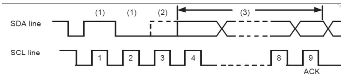
Figure 26-8 I 2 C 总线仲裁示例
