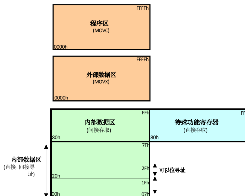
Figure 7-4 80C51地址空间
