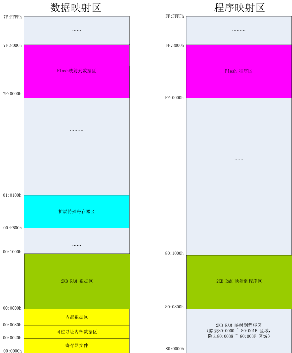
Figure 7-7 HC16Lxx 地址映射
