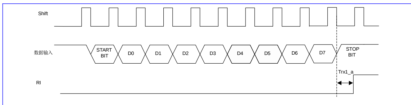
Figure 24-5 串行接收模式1
