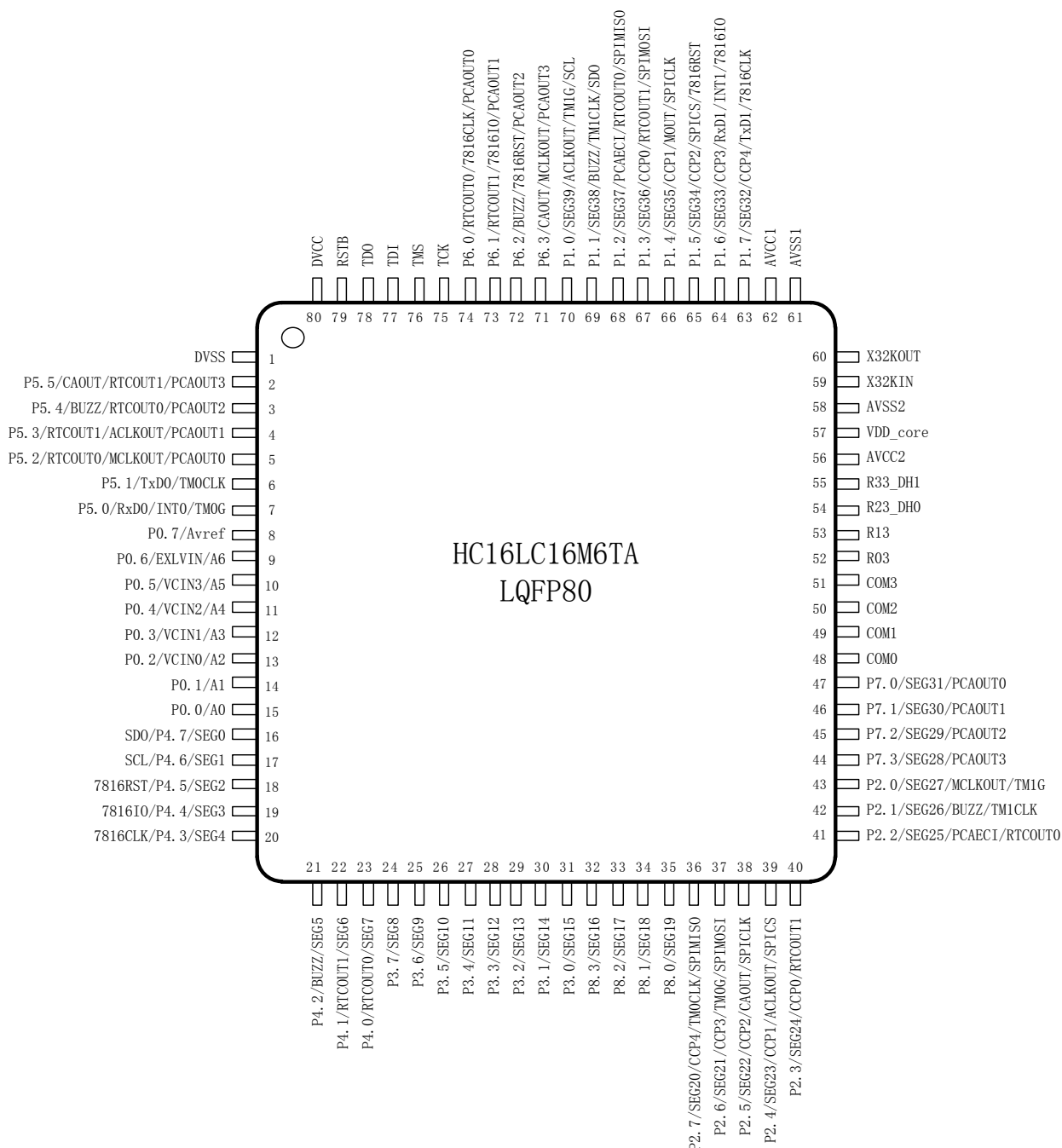
Figure 5-1 HC16LC16M6TA 80-pin 管脚定义
