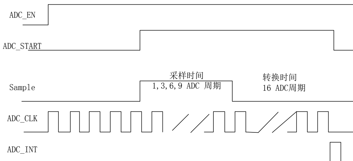
Figure 28-2 ADC单次采样过程
