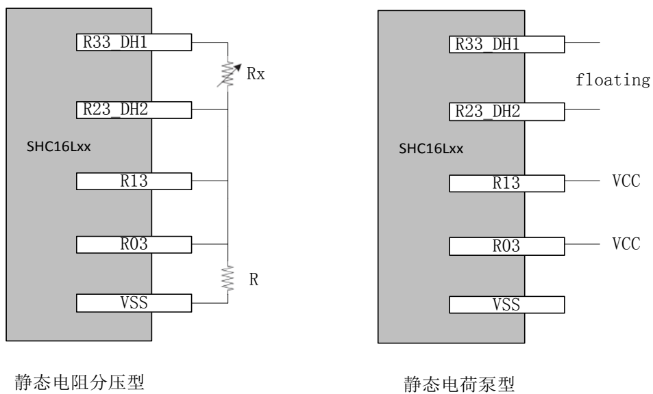
Figure 31-1 LCD 典型应用图
