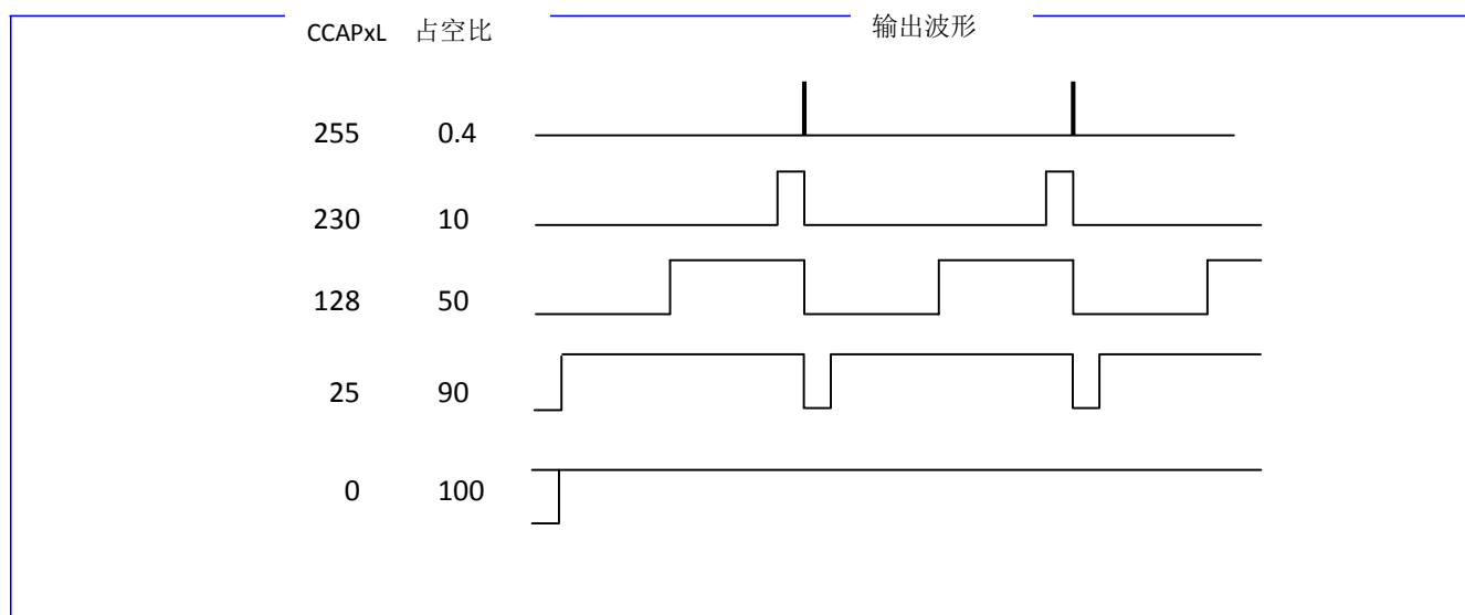
Figure 18-6 PWM 脉冲调制波形
