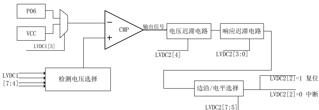
Figure 30-1 低电压检测器框架图
