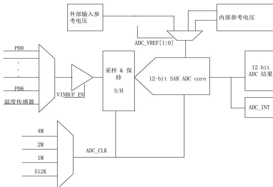
Figure 28-1 SARADC 框架图
