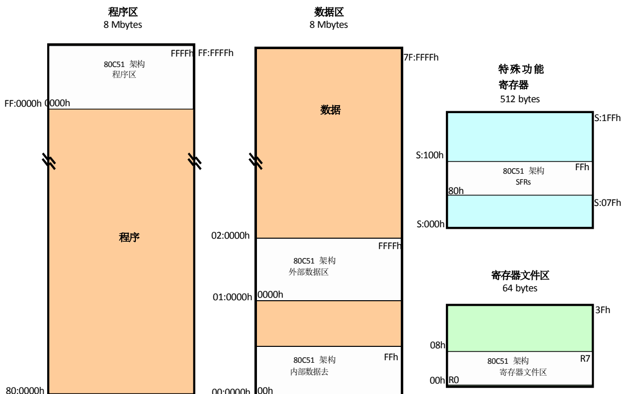
Figure 7-5 80C51 地址映射到80C251 架构
