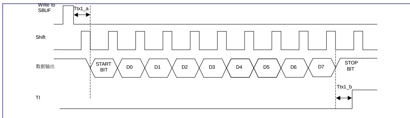
Figure 24-4 串口发送模式1
