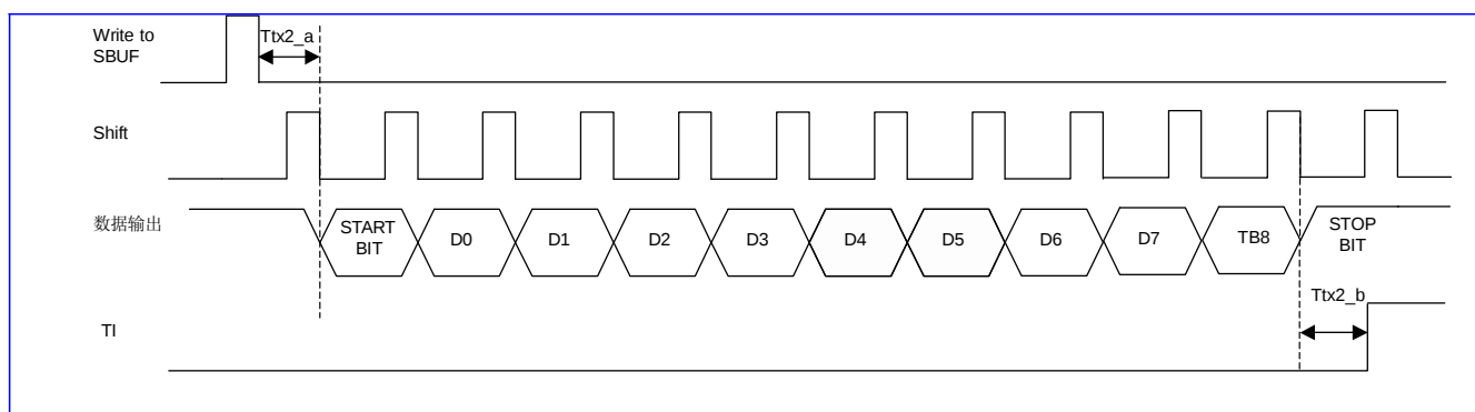
Figure 24-6 串口发送模式2
