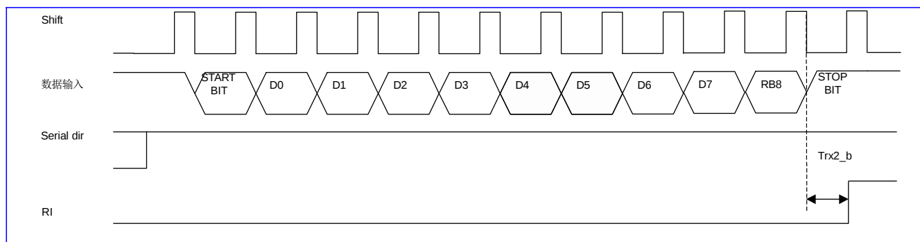
Figure 24-7 串口接收模式2
