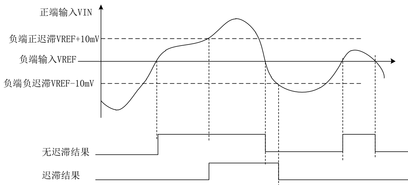
Figure 29-3 模拟比较器迟滞
